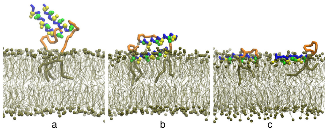
Fig. 8. Three simulation snapshots for two LP 12 E that are initially anchored at a short distance. From left to right: a) homo-dimer formation in solution; b) binding of one peptide and c) separation of the homo-dimer into individual lipopeptides that diffuse along the membrane surface. The color code is identical to the one in Fig. 3.
