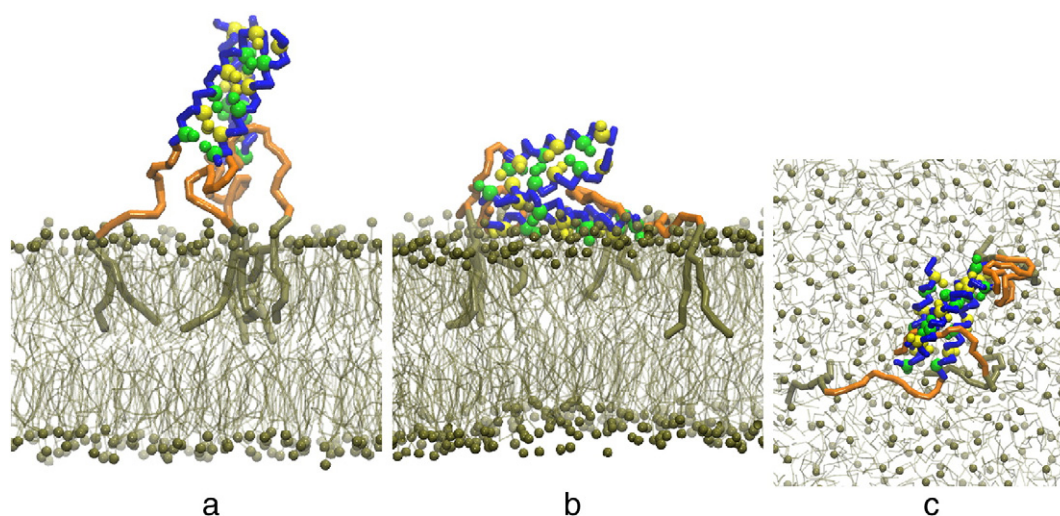
Fig. 9. Two simulation snapshots for four LP12E. From left to right: a) tetramer formation in solution; b) stable conformation after long (20 \mu s) simulation, with two lipopeptides of the original tetramer attached to the membrane surface and one homo-dimer in solution; c) top view of b). The color code is identical to the one in Fig. 3.
