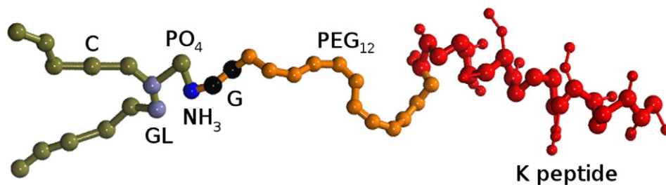
Fig. 1. The coarse-grained model of the lipo-peptide LP_{12}K . The lipid is depicted with tan tails and blue/tan/ice blue colored beads for the choline/phosphate/glycerol moieties. The PEG beads are orange and the succinic anhydride is black. The K peptide is represented with red beads, where the size indicates backbone (big) or side chain (small) particles. In the remainder, we use a blue bead representation for the E peptide.
